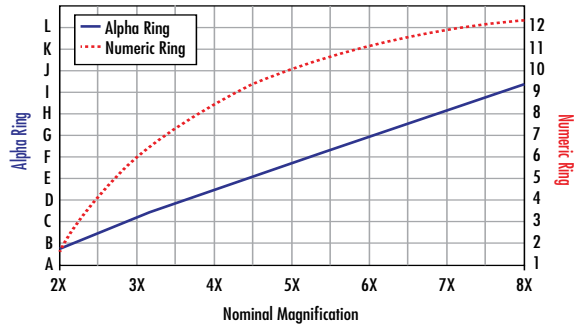
Variable Beam Expander Magnification Settings 2X-8X, VIS (#87-569)
