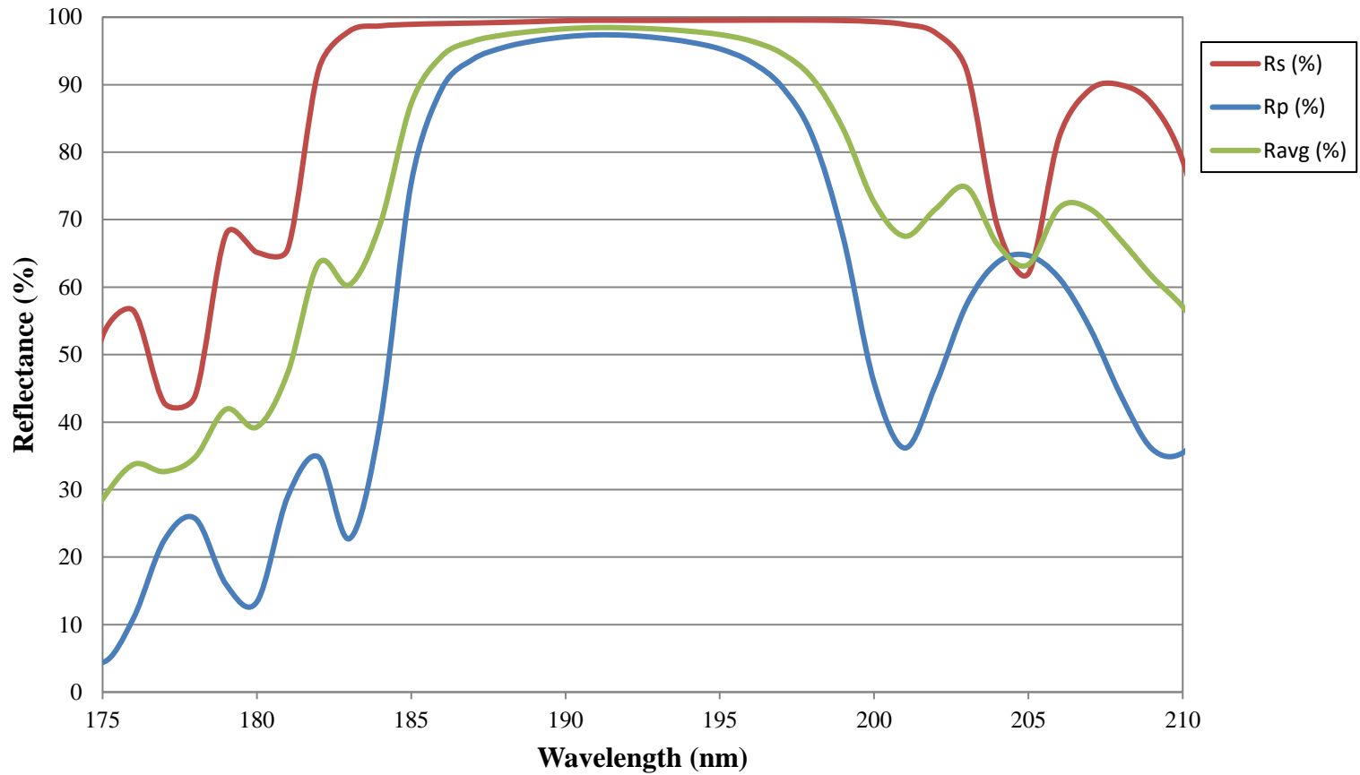
193nm 45° AOI - Excimer Laser Line Mirror Coating Performance FOR REFERENCE ONLY
