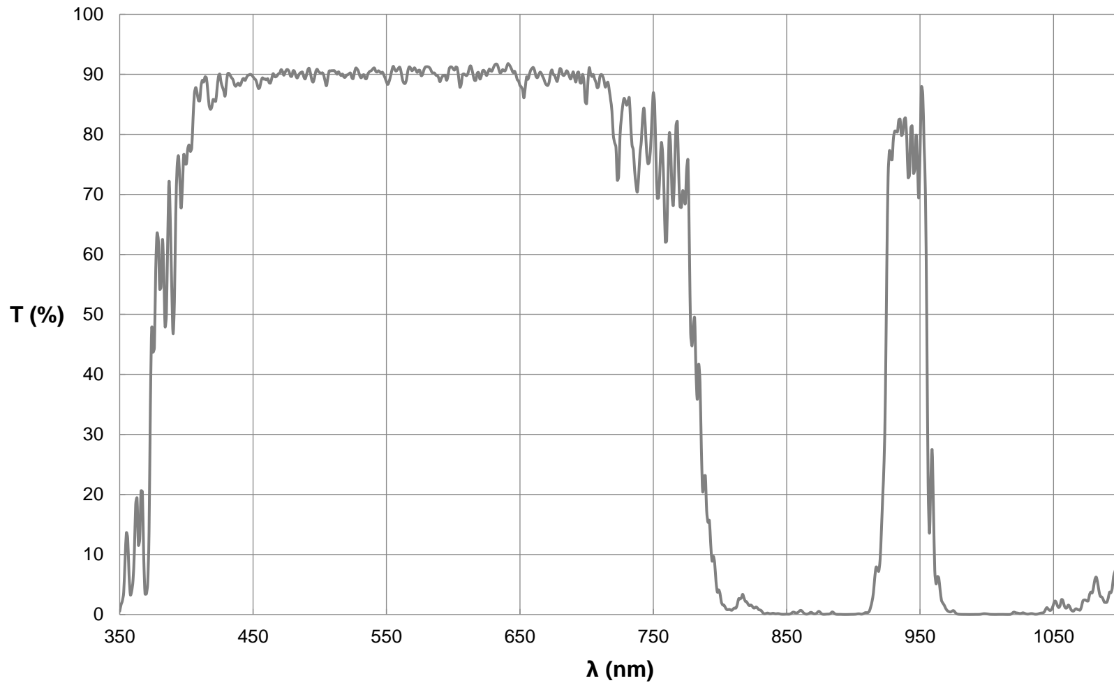
Everix Ultra-Thin Bandpass Filter, 940nm, OD 2.0 FOR REFERENCE ONLY
