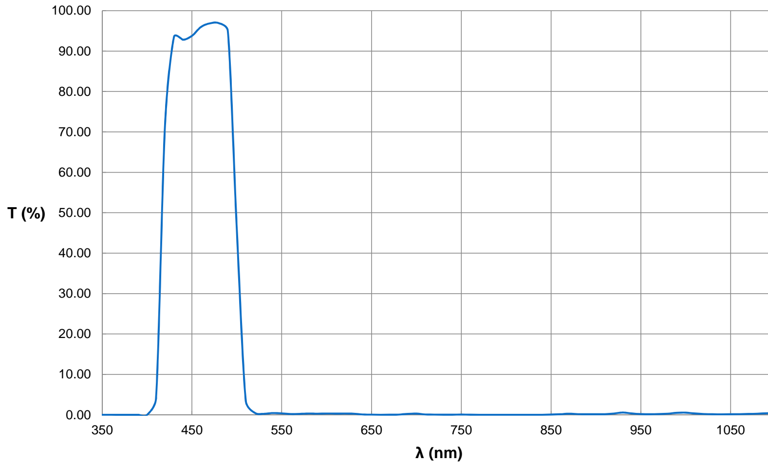
Blue Machine Vision Bandpass Filter, 470nm FOR REFERENCE ONLY
