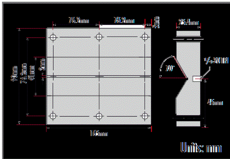
V-Block Base
