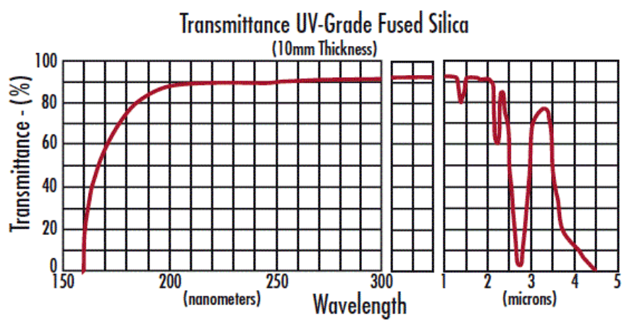
UV FS Transmission Curve
