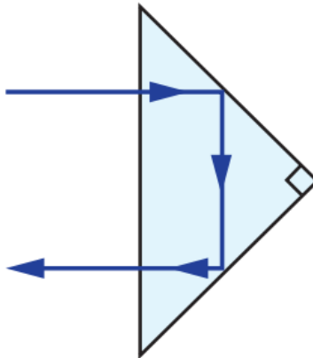
Right Angle Prism Ray Path
