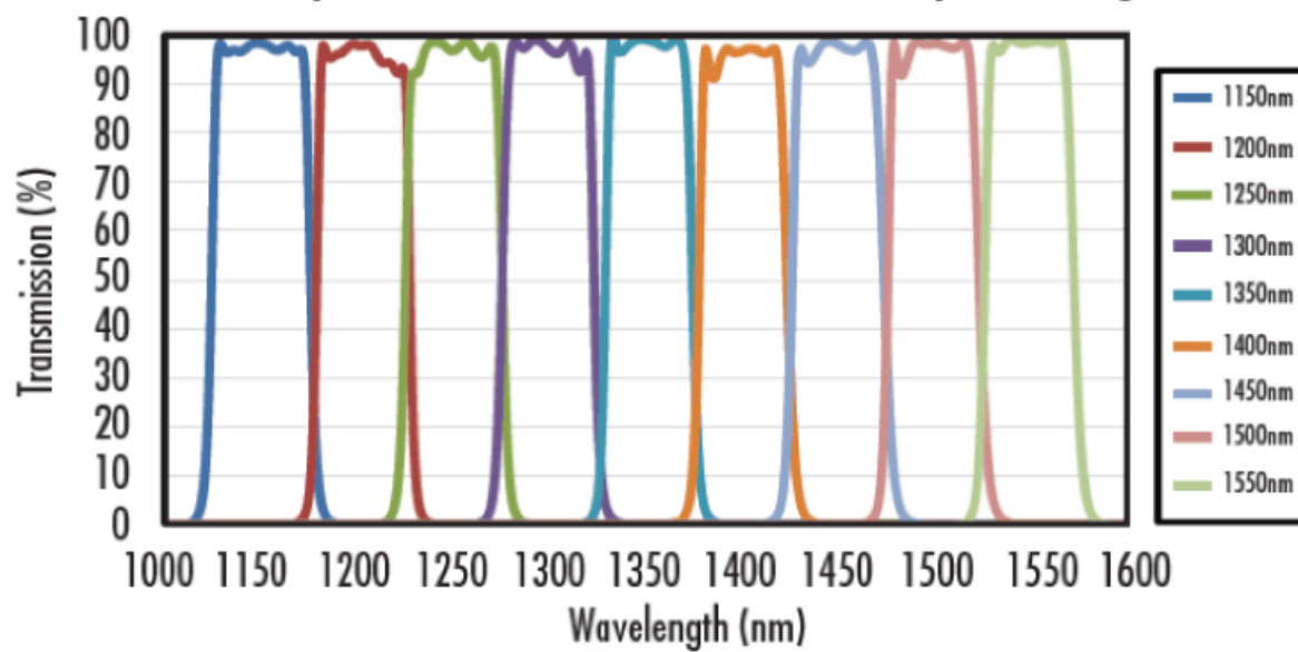
50nm Bandpass Filter Kit Curve 1150 - 1550nm Spectral Range
