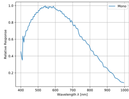
IMX546 Sensor QE Curve
