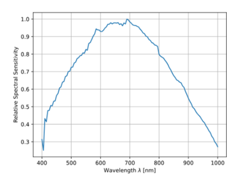
IMX900 Sensor QE Curve
