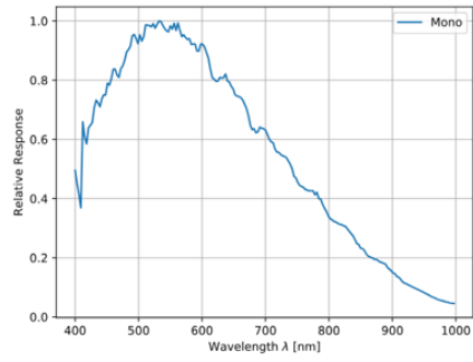
GMAX2518 Sensor QE Curve
