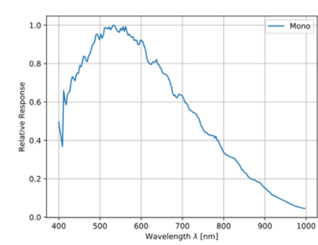
GMAX2505 Sensor QE Curve
