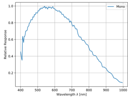
IMX547 Sensor QE Curve
