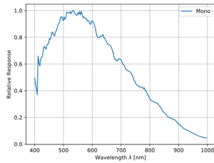
GMAX2509 Sensor QE Curve
