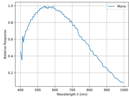
E2525A Sensor QE Curve
