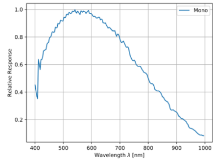
IMX545 Sensor QE Curve
