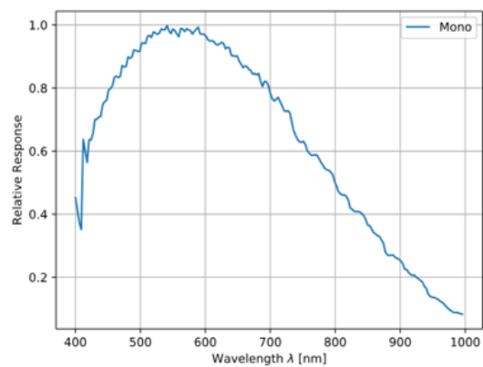
IMX547 Sensor QE Curve
