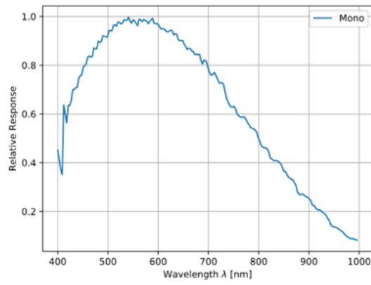
IMX545 Sensor QE Curve
