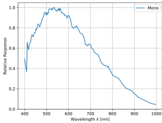
GMAX2509 Sensor QE Curve
