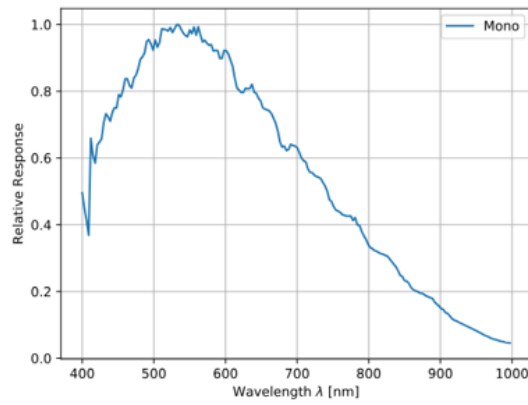
GMAX2518 Sensor QE Curve
