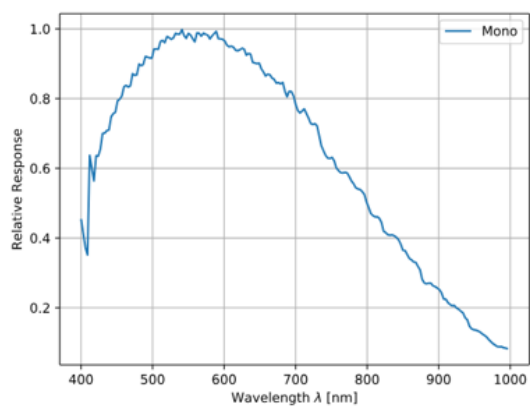
E2525A Sensor QE Curve
