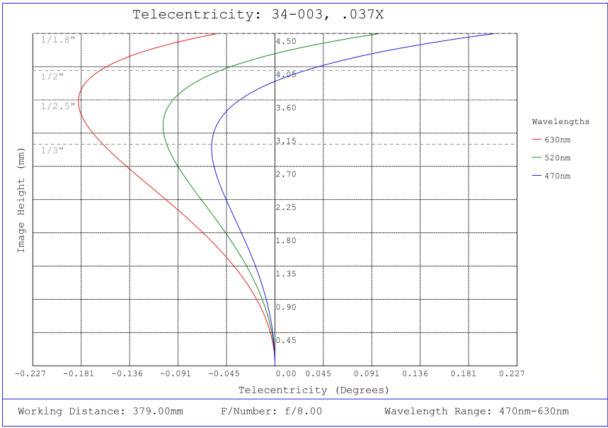
#34-003, 0.037X, 1/1.8" C-Mount TitanTL® Telecentric Lens, Telecentricity Plot
