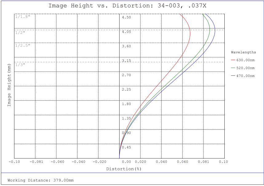
#34-003, 0.037X, 1/1.8" C-Mount TitanTL® Telecentric Lens, Distortion Plot
