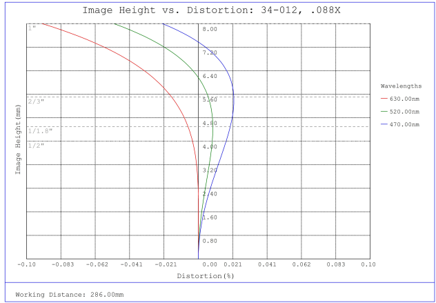
#34-012, 0.088X, 1" C-Mount TitanTL® Telecentric Lens, Distortion Plot
