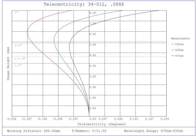
#34-012, 0.088X, 1" C-Mount TitanTL® Telecentric Lens, Telecentricity Plot
