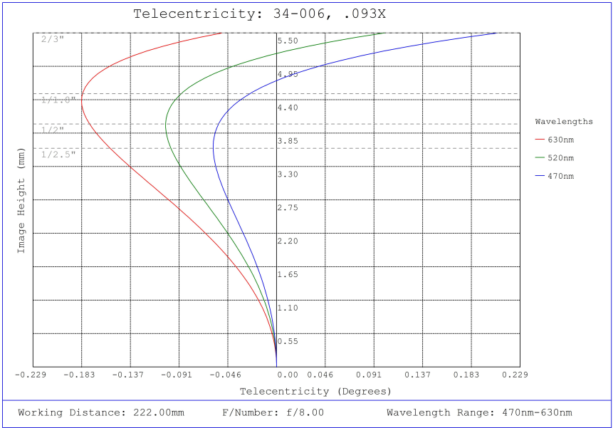
#34-006, 0.093X, 2/3" C-Mount TitanTL® Telecentric Lens, Telecentricity Plot
