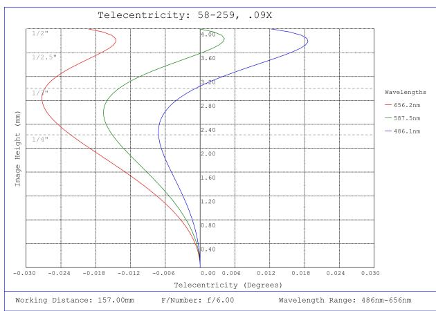
#58-259, 0.09X 1/2" GoldTL™ Telecentric Lens, Telecentricity Plot
