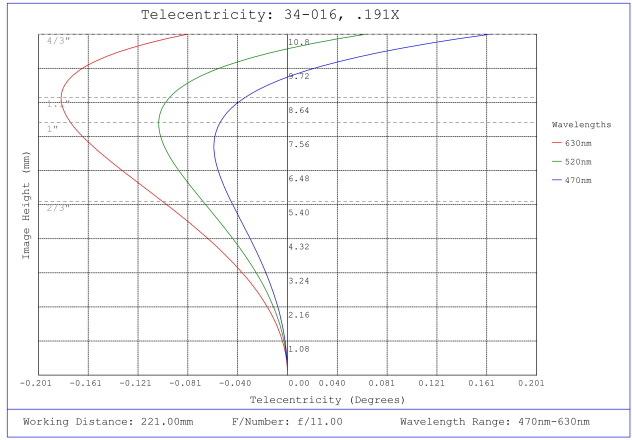
#34-016, 0.191X, 4/3" C-Mount TitanTL® Telecentric Lens, Telecentricity Plot
