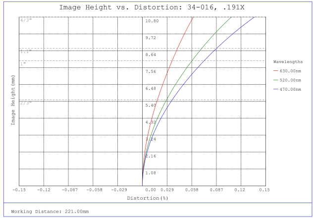
#34-016, 0.191X, 4/3" C-Mount TitanTL® Telecentric Lens, Distortion Plot
