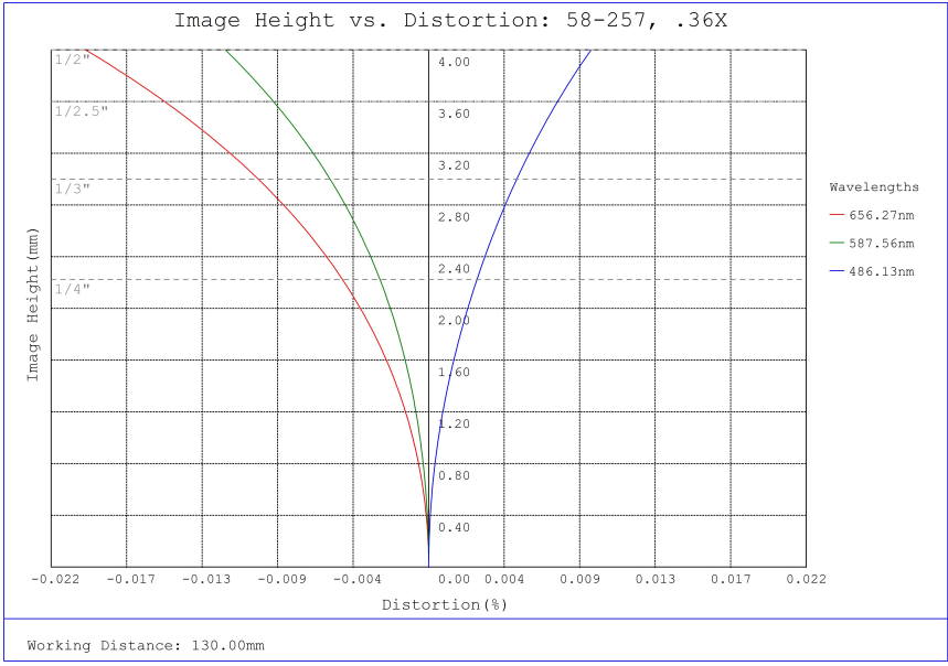
#58-257, 0.36X ½" GoldTL™ Telecentric Lens, Distortion Plot
