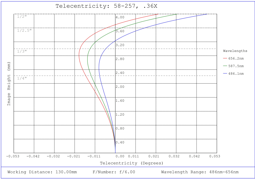
#58-257, 0.36X ½" GoldTL™ Telecentric Lens, Telecentricity Plot
