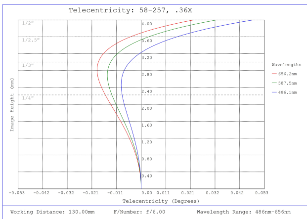
#58-257, 0.36X 1/2" GoldTL™ Telecentric Lens, Telecentricity Plot
