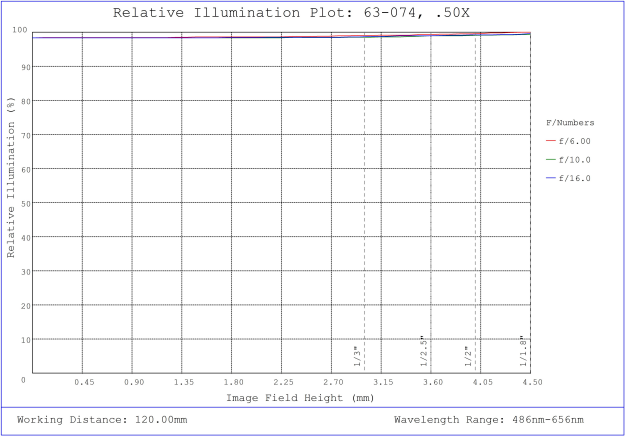
#63-074, 0.50X SilverTL™ Telecentric Lens, Relative Illumination Plot
