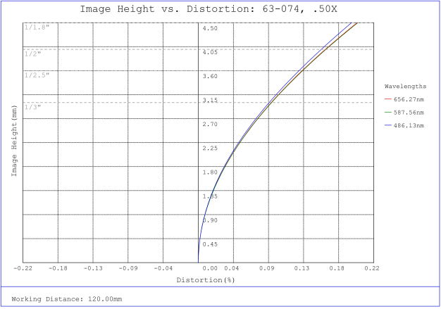
#63-074, 0.50X SilverTL™ Telecentric Lens, Distortion Plot
