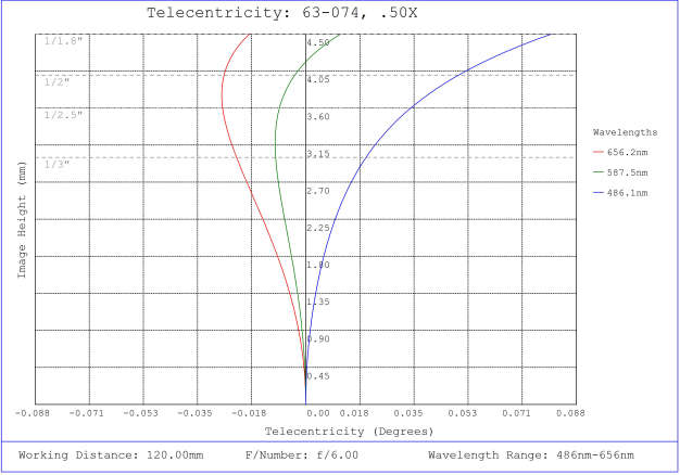
#63-074, 0.50X SilverTL™ Telecentric Lens, Telecentricity Plot
