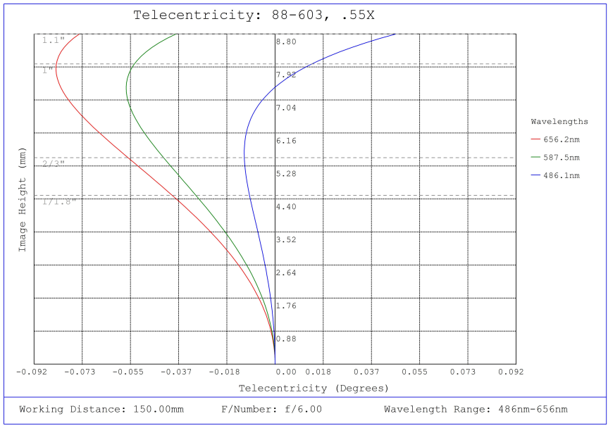
#88-603, 0.55X CobaltTL Telecentric Lens, Telecentricity Plot
