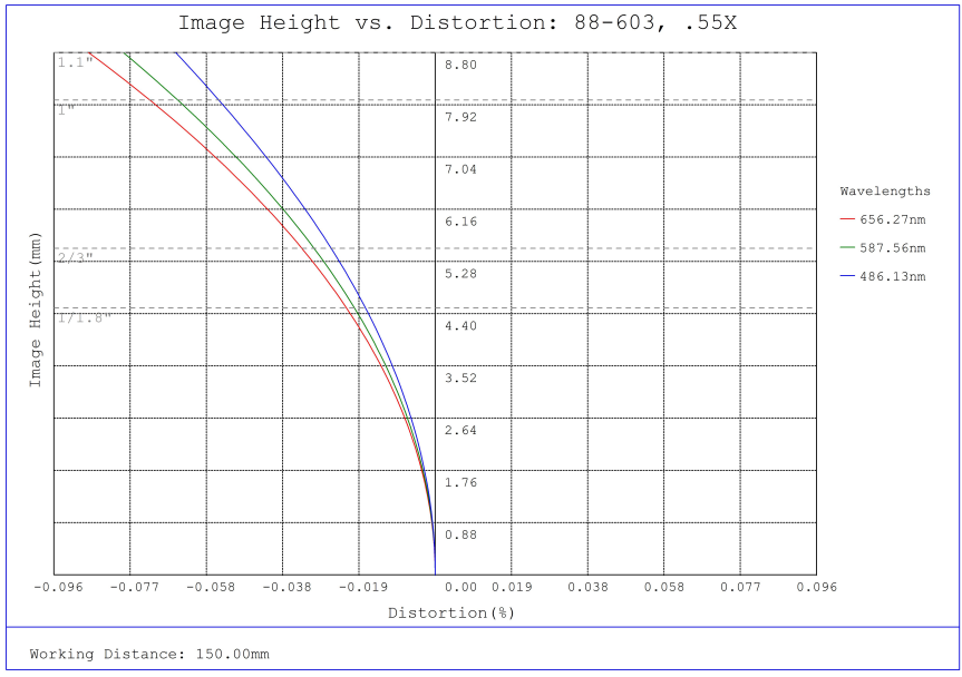
#88-603, 0.55X CobaltTL Telecentric Lens, Distortion Plot
