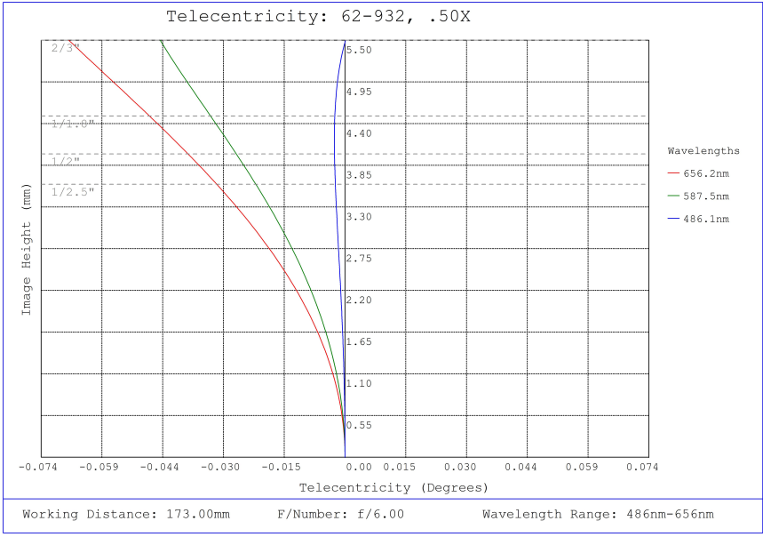
#62-932, 0.5X, 2/3" C-Mount PlatinumTL™ Telecentric Lens, Telecentricity Plot
