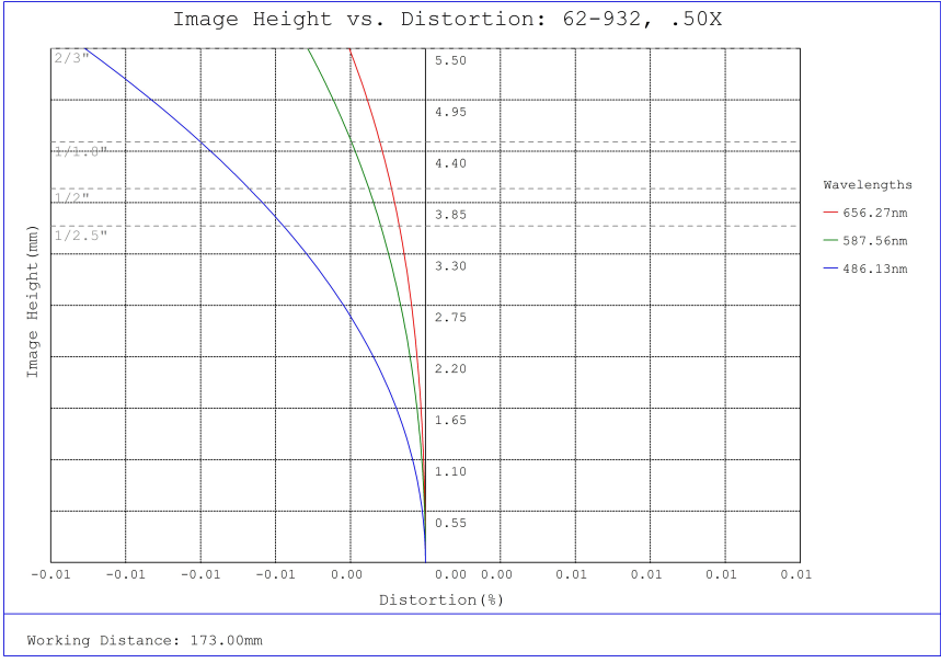
#62-932, 0.5X, 2/3" C-Mount PlatinumTL™ Telecentric Lens, Distortion Plot
