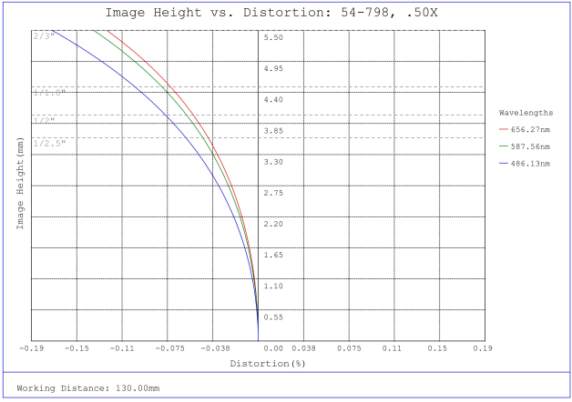
#54-798, 0.5X 2/3" GoldTL™ Telecentric Lens, Distortion Plot
