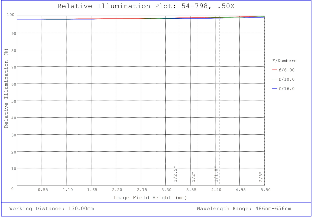
#54-798, 0.5X 2/3" GoldTL™ Telecentric Lens, Relative Illumination Plot
