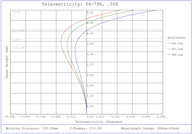
#54-798, 0.5X 2/3" GoldTL™ Telecentric Lens, Telecentricity Plot
