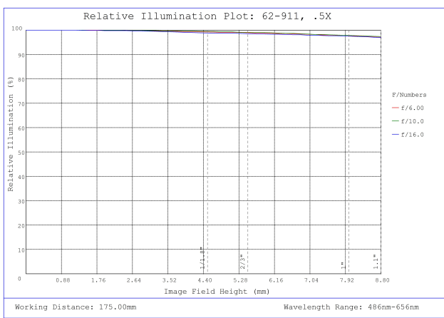
#62-911, 0.5X CobaltTL Telecentric Lens, Relative Illumination Plot
