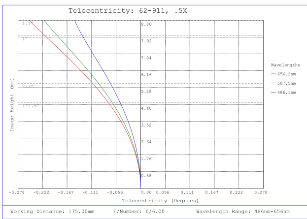
#62-911, 0.5X CobaltTL Telecentric Lens, Telecentricity Plot
