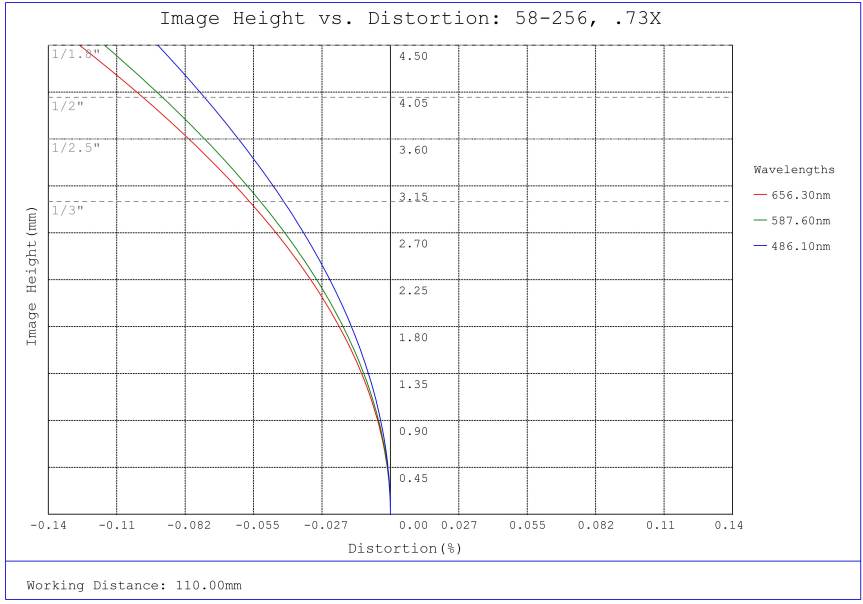
#58-256, 0.73X ½" GoldTL™ Telecentric Lens, Distortion Plot
