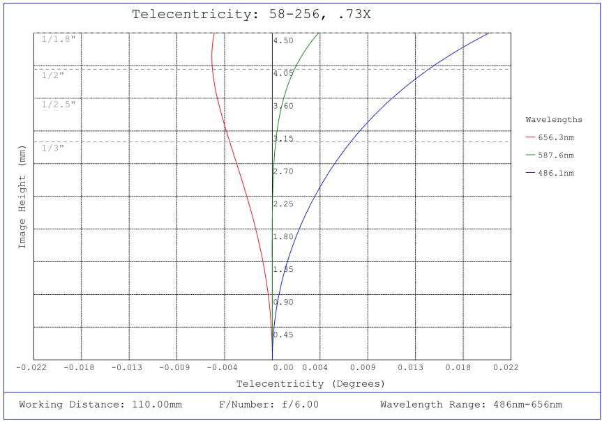
#58-256, 0.73X ½" GoldTL™ Telecentric Lens, Telecentricity Plot
