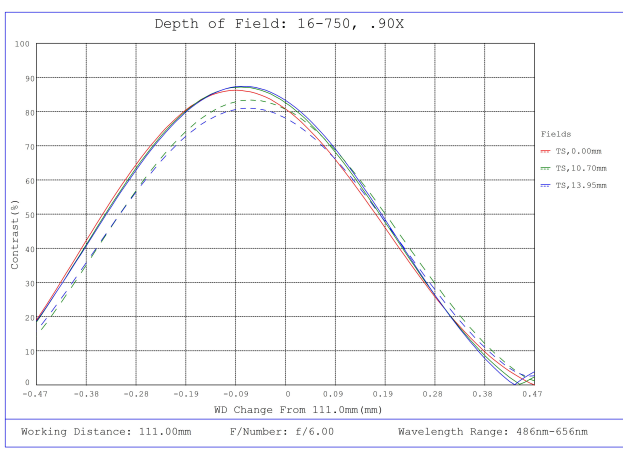
#16-750, 0.9X, 28.7mm TFL-Mount PlatinumTL™ Telecentric Lens, Depth of Field Plot, 111mm Working Distance, f6
