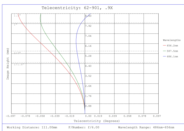
#62-901, 0.9X CobaltTL Telecentric Lens, Telecentricity Plot
