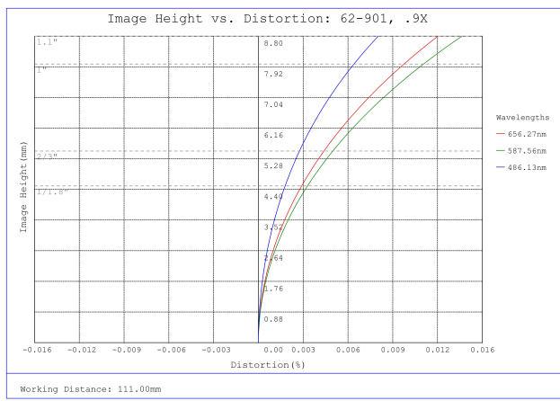
#62-901, 0.9X CobaltTL Telecentric Lens, Distortion Plot
