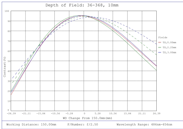
#36-368, 10mm FL f/2.5, Rugged Blue Series M12 Lens, Depth of Field Plot, 150mm Working Distance, f2.5
