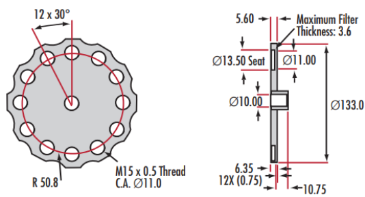
12-Position Filter Wheel Assembly
