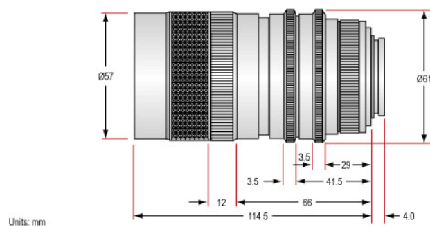
Manual Zoom Video Lens #53-153
