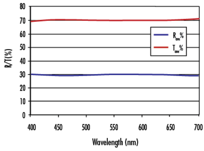
VIS 30R/70T Beamsplitter
