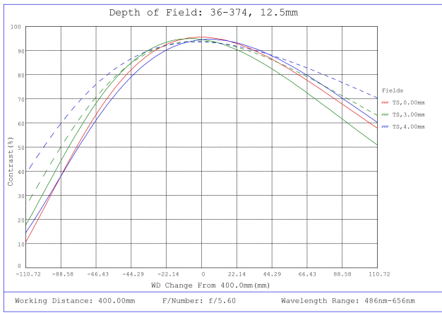
#36-374, 12.5mm FL f/5.6, Rugged Blue Series M12 Lens, Depth of Field Plot, 400mm Working Distance, f5.6
