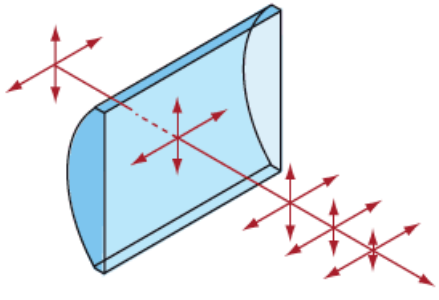
PCX Rectangular
