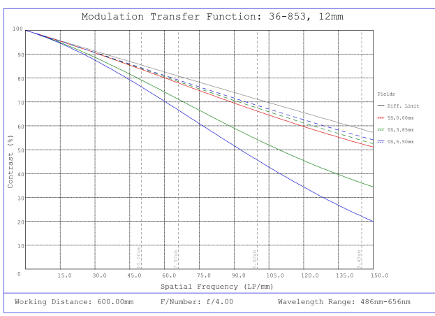
#36-853, 12mm f/4, 400-2000mm Primary WD, HRr Series Fixed Focal Length Lens, Modulated Transfer Function (MTF) Plot, 600mm Working Distance, f4
