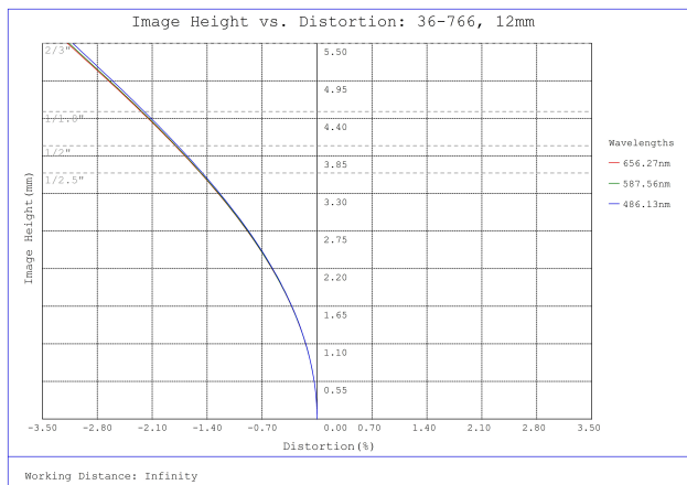
#36-766, 12mm f/8, 150-500mm Primary WD, HRi Series Fixed Focal Length Lenses, Distortion Plot
