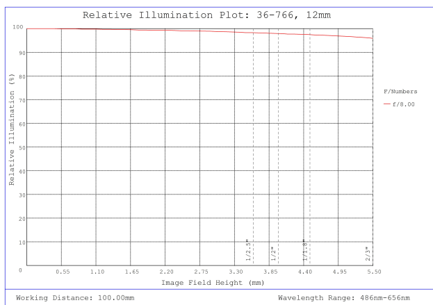
#36-766, 12mm f/8, 150-500mm Primary WD, HRi Series Fixed Focal Length Lenses, Relative Illumination Plot
