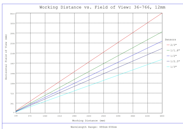
#36-766, 12mm f/8, 150-500mm Primary WD, HRi Series Fixed Focal Length Lenses, Working Distance versus Field of View Plot
