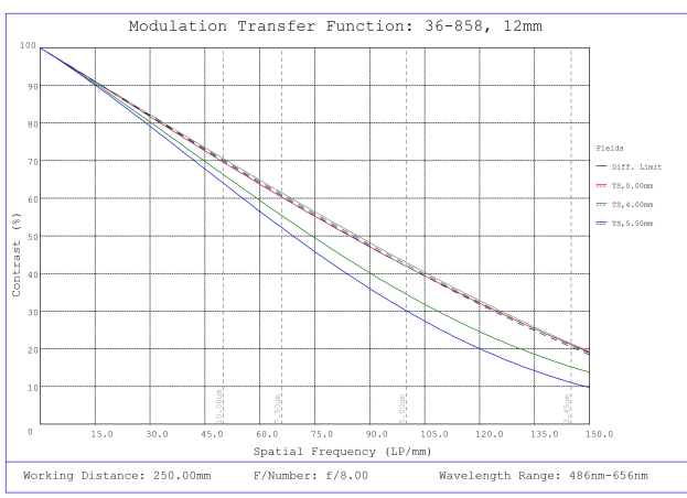
#36-858, 12mm f/8, 150-500mm Primary WD, HRr Series Fixed Focal Length Lens, Modulated Transfer Function (MTF) Plot, 250mm Working Distance, f8
