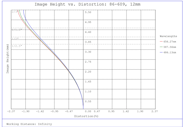
#86-609, 12mm, f/4 Ci Series Fixed Focal Length Lens, Distortion Plot
