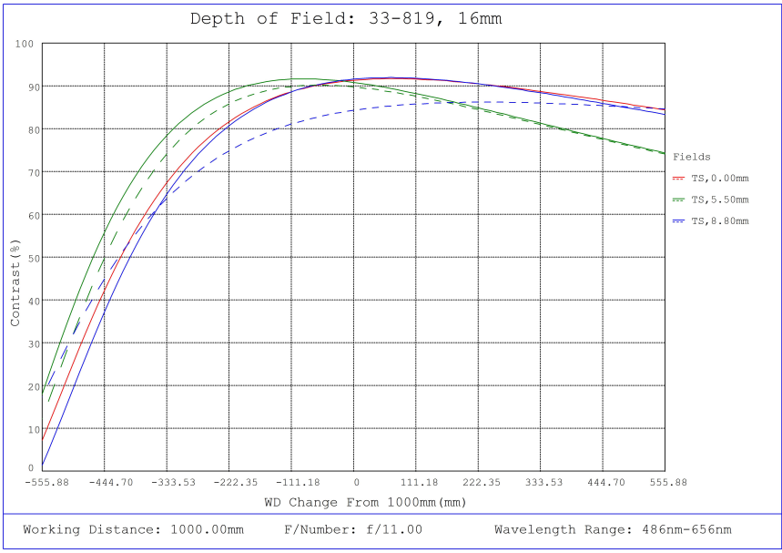
#33-819, 16mm f/11, HPi Series Fixed Focal Length Lens, Depth of Field Plot, 1000mm Working Distance, f11
