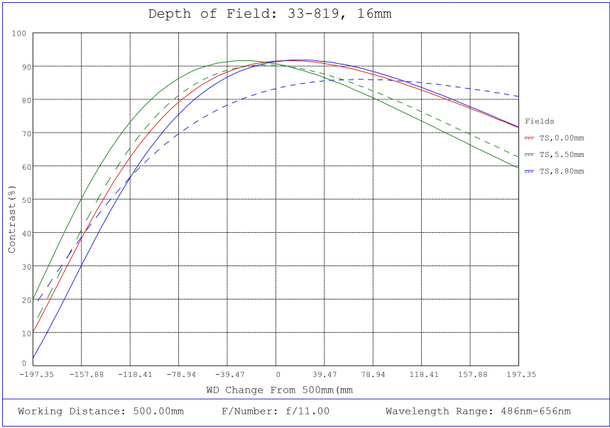
#33-819, 16mm f/11, HPi Series Fixed Focal Length Lens, Depth of Field Plot, 500mm Working Distance, f11
