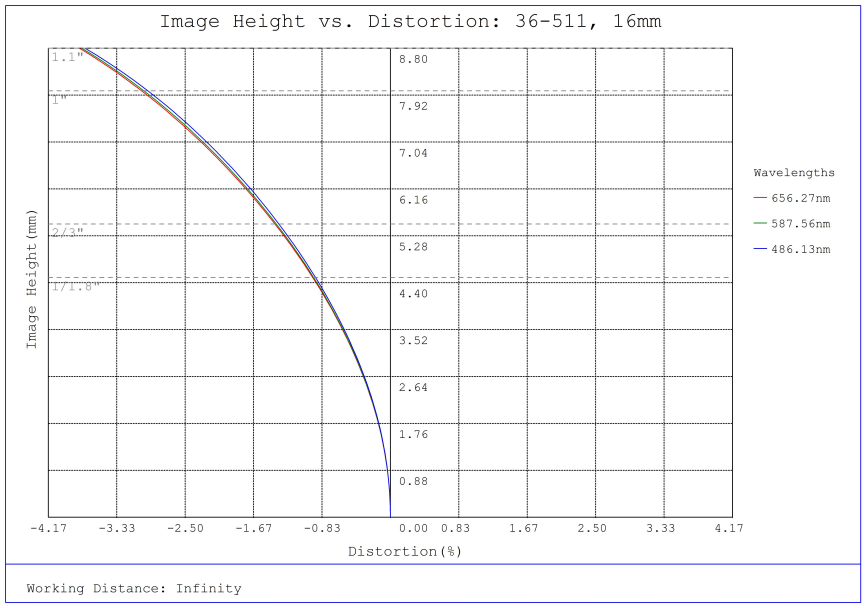
#36-511, 16mm f/1.8, HPr Series Fixed Focal Length Lens, Distortion Plot
