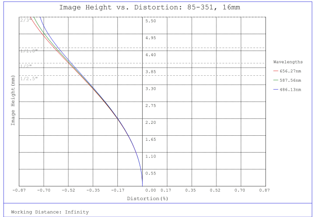
#85-351, 16mm, f/4 Ci Series Fixed Focal Length Lens, Distortion Plot
