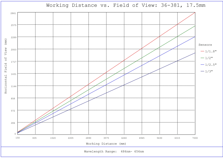
#36-381, 17.5mm FL f/4, Rugged Blue Series M12 Lens, Working Distance versus Field of View Plot
