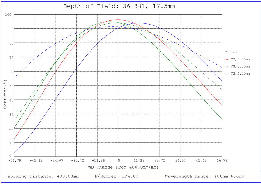
#36-381, 17.5mm FL f/4, Rugged Blue Series M12 Lens, Depth of Field Plot, 400mm Working Distance, f4
