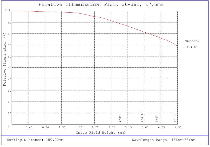
#36-381, 17.5mm FL f/4, Rugged Blue Series M12 Lens, Relative Illumination Plot
