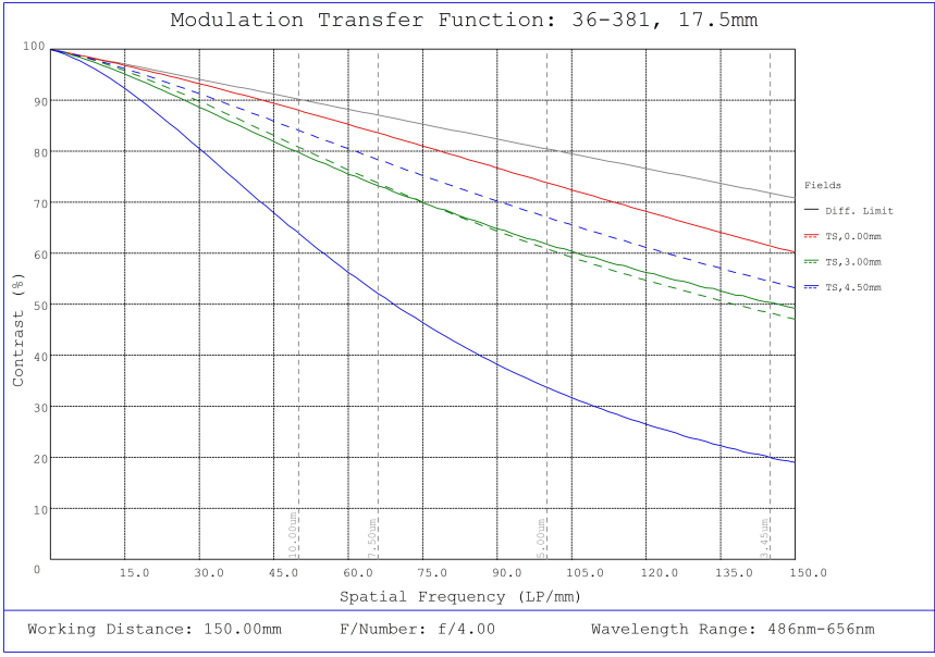
#36-381, 17.5mm FL f/4, Rugged Blue Series M12 Lens, Modulated Transfer Function (MTF) Plot, 150mm Working Distance, f4
