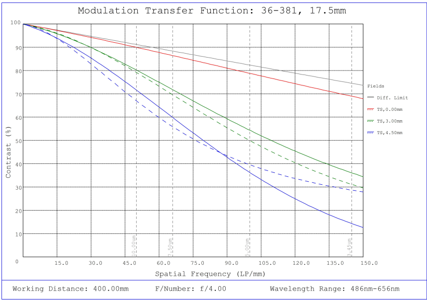
#36-381, 17.5mm FL f/4, Rugged Blue Series M12 Lens, Modulated Transfer Function (MTF) Plot, 400mm Working Distance, f4
