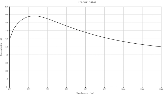
1.7mm FL, f/4, Low Distortion M12 Lens, Transmission Plot
