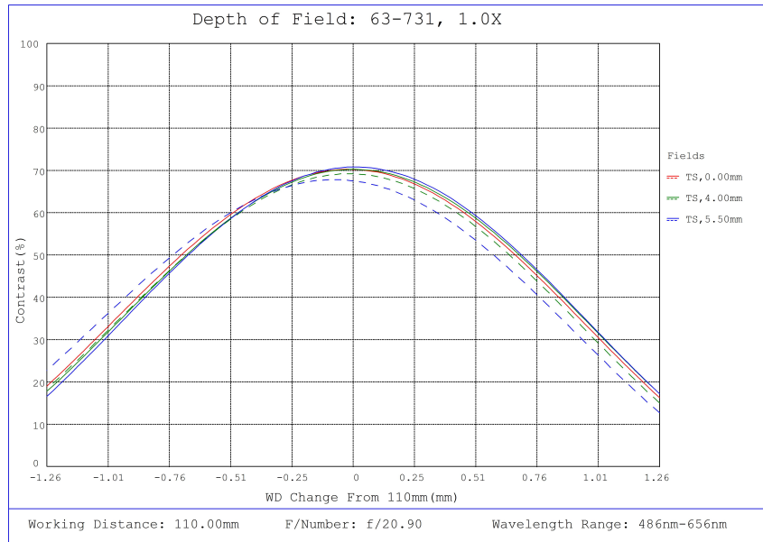
#63-731, 1X, 110mm WD CompactTL™ Telecentric Lens, Depth of Field Plot, 110mm Working Distance, f20.9
