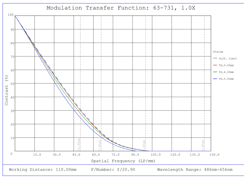
#63-731, 1X, 110mm WD CompactTL™ Telecentric Lens, Modulated Transfer Function (MTF) Plot, 110mm Working Distance, f20.9
