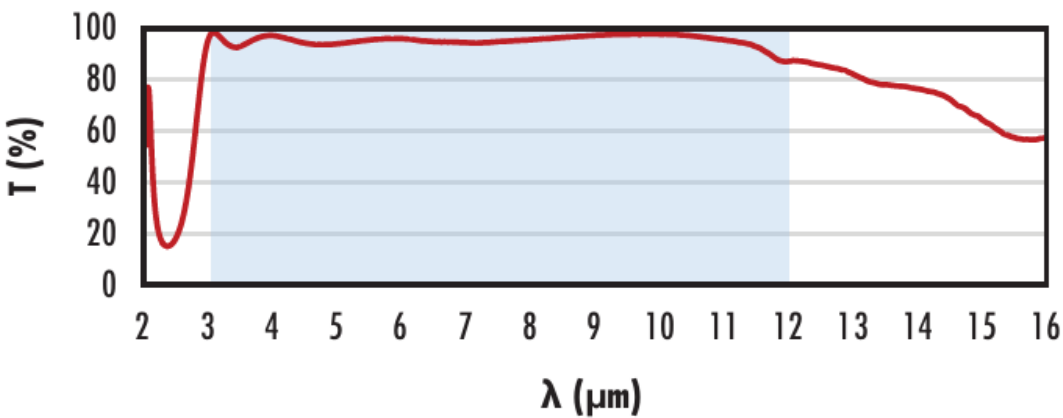
Ge with 3-12µm AR Coating Typical Transmission
