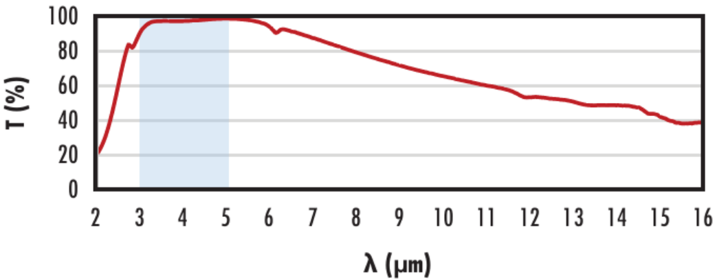
Ge with 3-5µm AR Coating Typical Transmission
