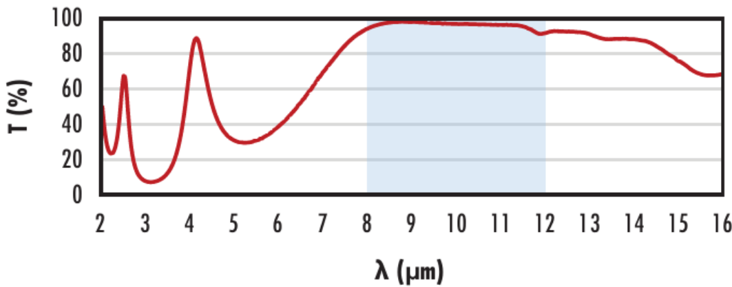
8-12µm AR Coated Germanium Typical Transmission
