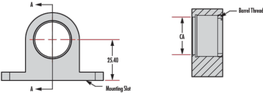
Side Flange Type (#36-414 & #36-418)
