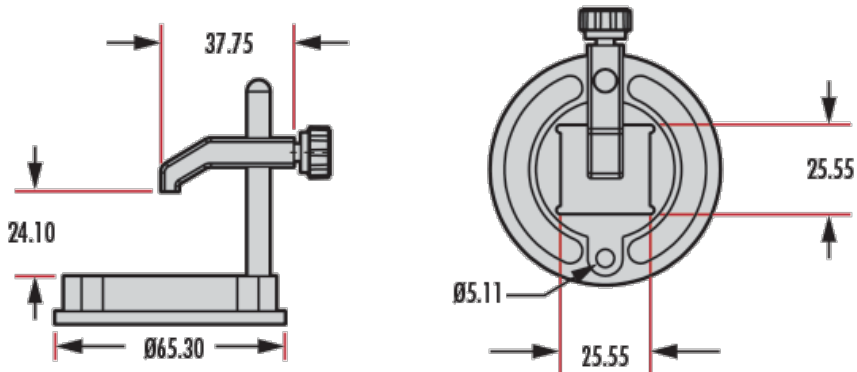
Cube Beamsplitter Type (#36-415)
