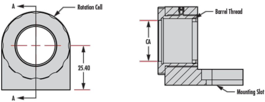
L-Slot Type (#36-411 & #36-417) Optic Rotation
