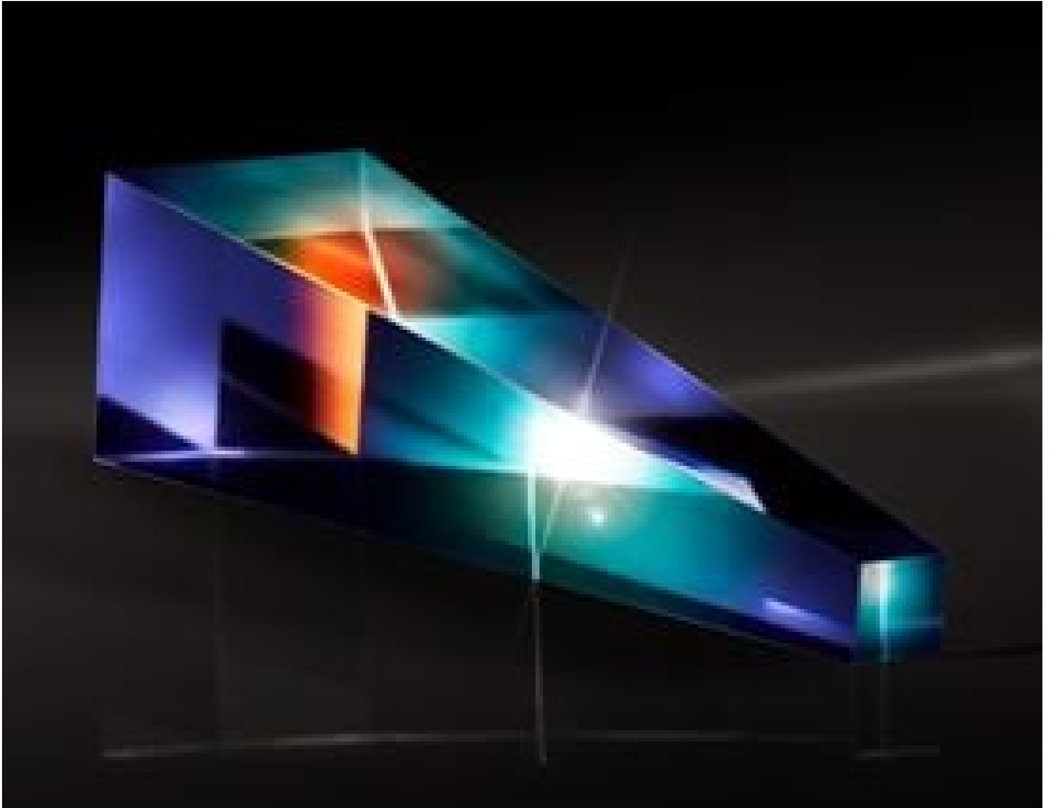
TECHSPEC® Tapered Light Pipe Homogenizing Rods
