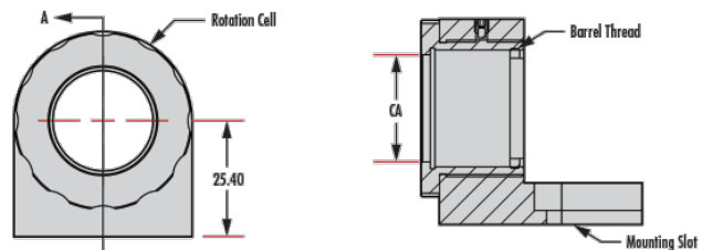
L-Slot Type (#36-411 & #36-417) Optic Rotation
