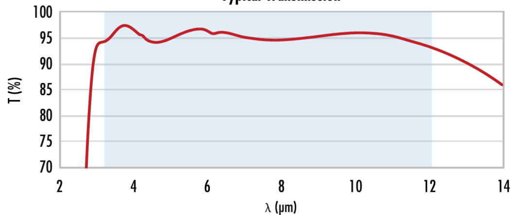
ZnSe with 3-12µm AR Coating Typical Transmission
