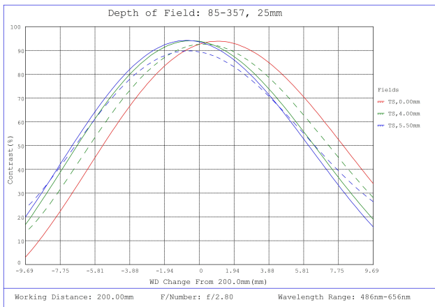
#85-357, 25mm, f/2.8 Ci Series Fixed Focal Length Lens, Depth of Field Plot, 200mm Working Distance, f2.8
