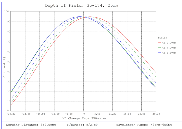
#35-174, 25mm, f/2.8 Cr Series Fixed Focal Length Lens, Depth of Field Plot, 350mm Working Distance, f2.8
