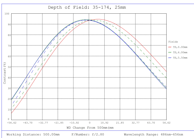
#35-174, 25mm, f/2.8 Cr Series Fixed Focal Length Lens, Depth of Field Plot, 500mm Working Distance, f2.8
