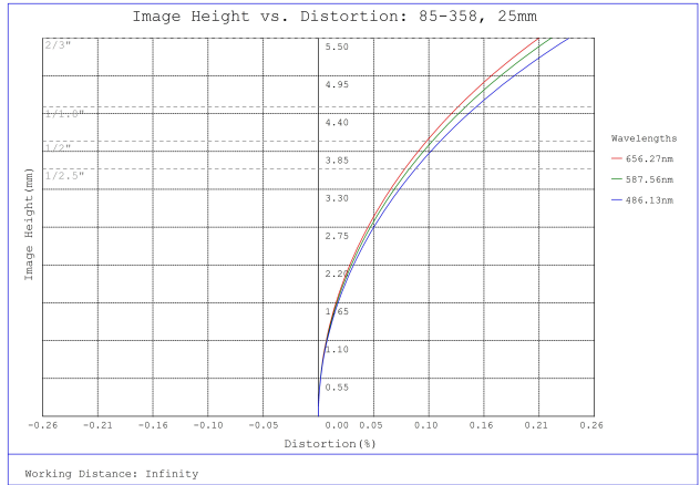
#85-358, 25mm, f/4 Ci Series Fixed Focal Length Lens, Distortion Plot
