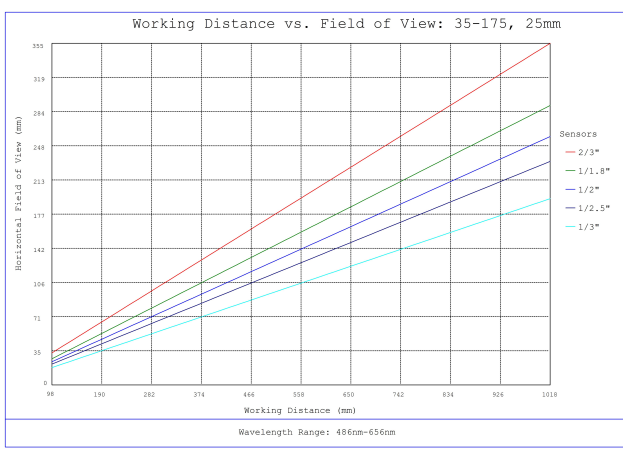
#35-175, 25mm, f/4 Cr Series Fixed Focal Length Lens, Working Distance versus Field of View Plot
